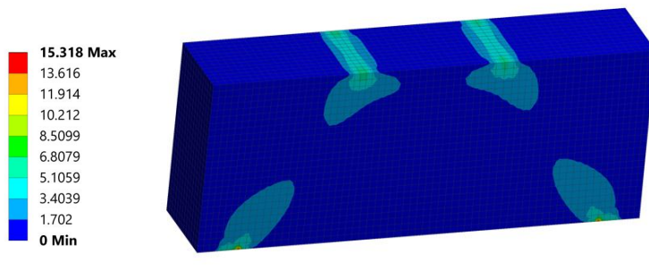
Fig:13b. Equivalent stress diagram of B1-0.67-140
