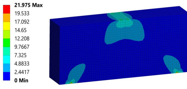
Fig:13d. Equivalent stress diagram of B1-1-140
